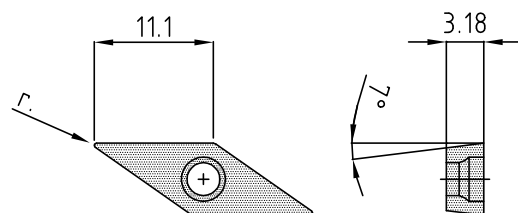
VCGW..N-FA-G6A
