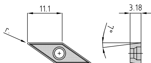
VCMT..N-FA-G5D
