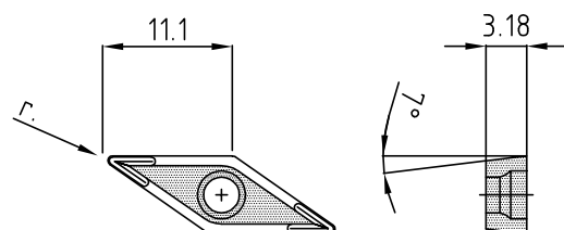
VCMT..N-FM-G5D
